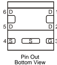
U-DFN2020-6
